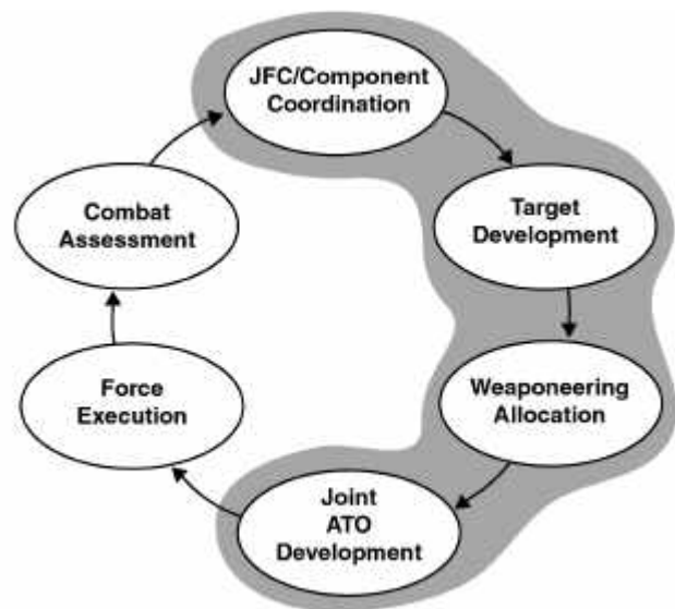
Figure 4-9. GAT Interaction.
