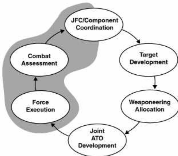
Figure 4-10. TAGS Interaction.
