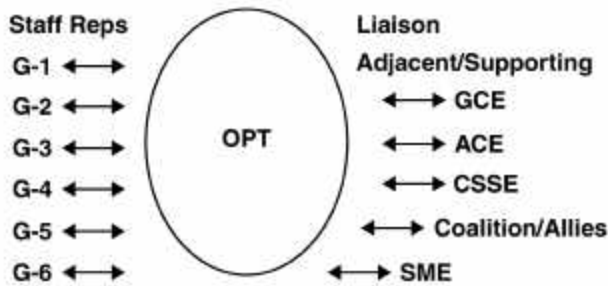
Figure 4-1. Appropriate Representation.
