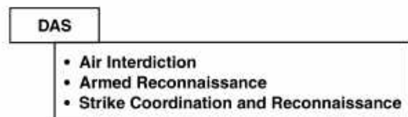
Figure 2-2. DAS Missions.
