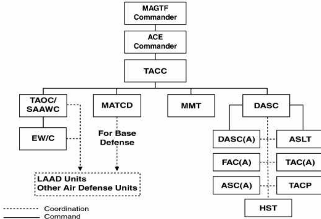
Figure 3-1. MACCS Organization.
